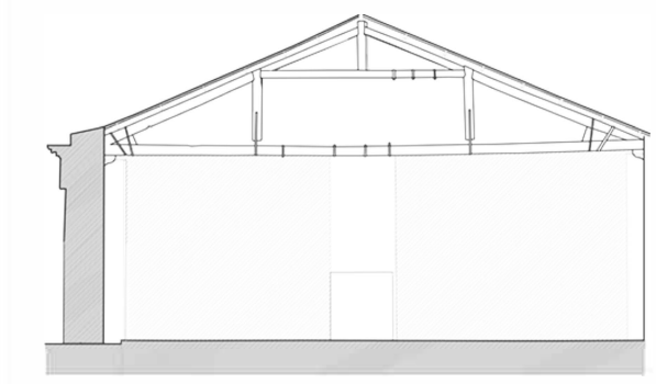
CROSS SECTION C-C'
